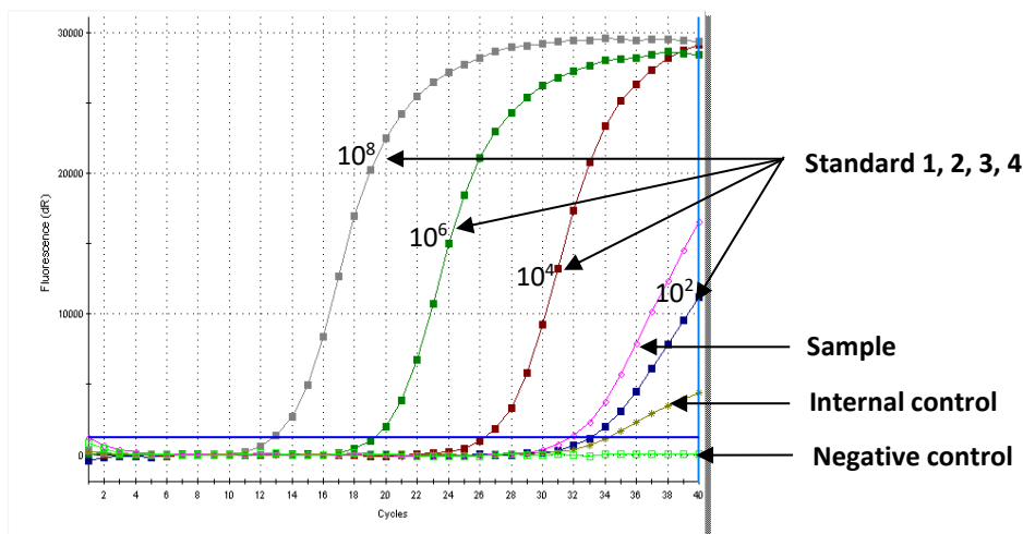
Amplification Plots
