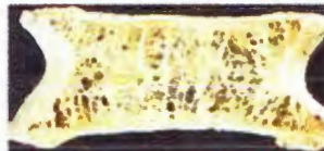
Osteopenia
